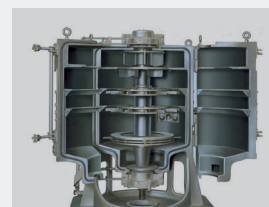
Vertical Mill
